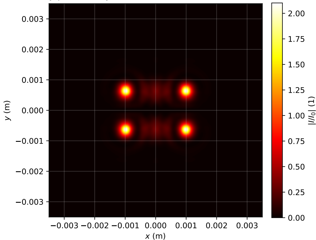
Intensity profile I(x, y, z = 1.672)/I_0 , P_{in}=5.0P_{cr} , artificial time
